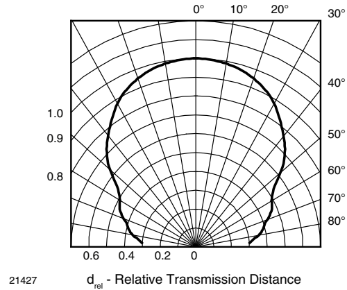
21427 d_{rel} - Relative Transmission Distance Fig. 12 - Horizontal Directivity
