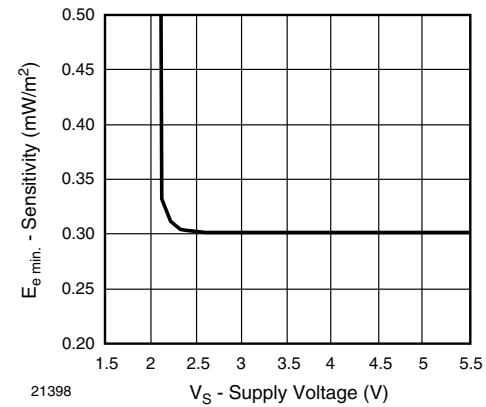
21398 V_S - Supply Voltage (V) Fig. 14 - Sensitivity vs. Supply Voltage
