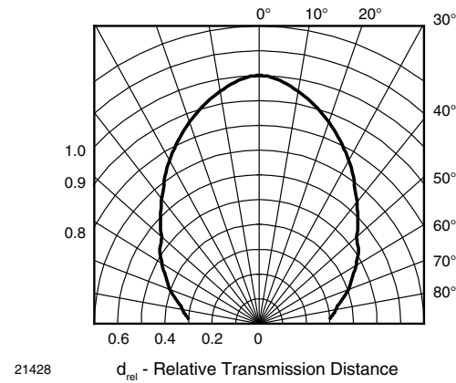
21428 d_{rel} - Relative Transmission Distance Fig. 13 - Vertical Directivity
